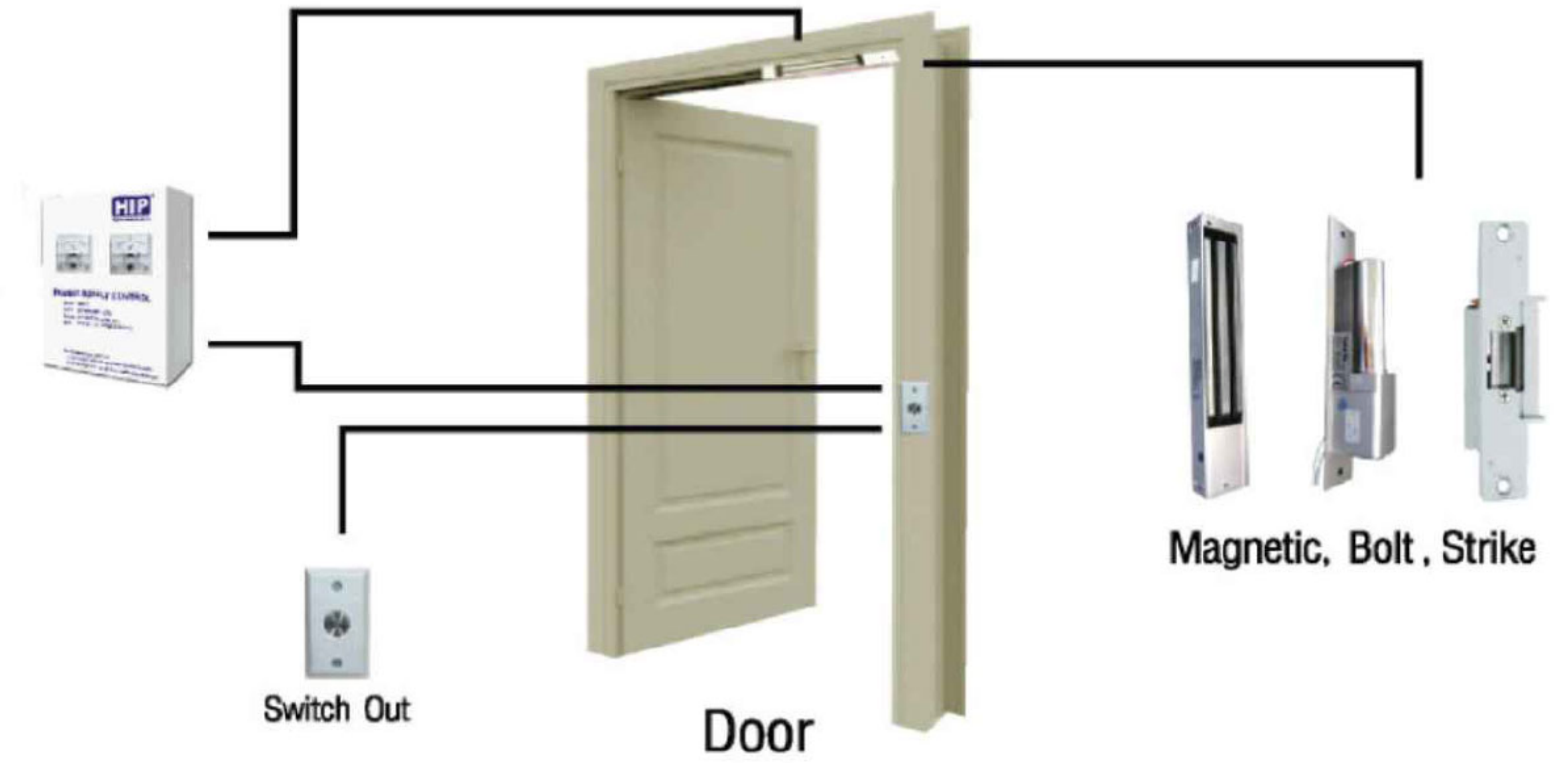
Connection Type Access Control System
