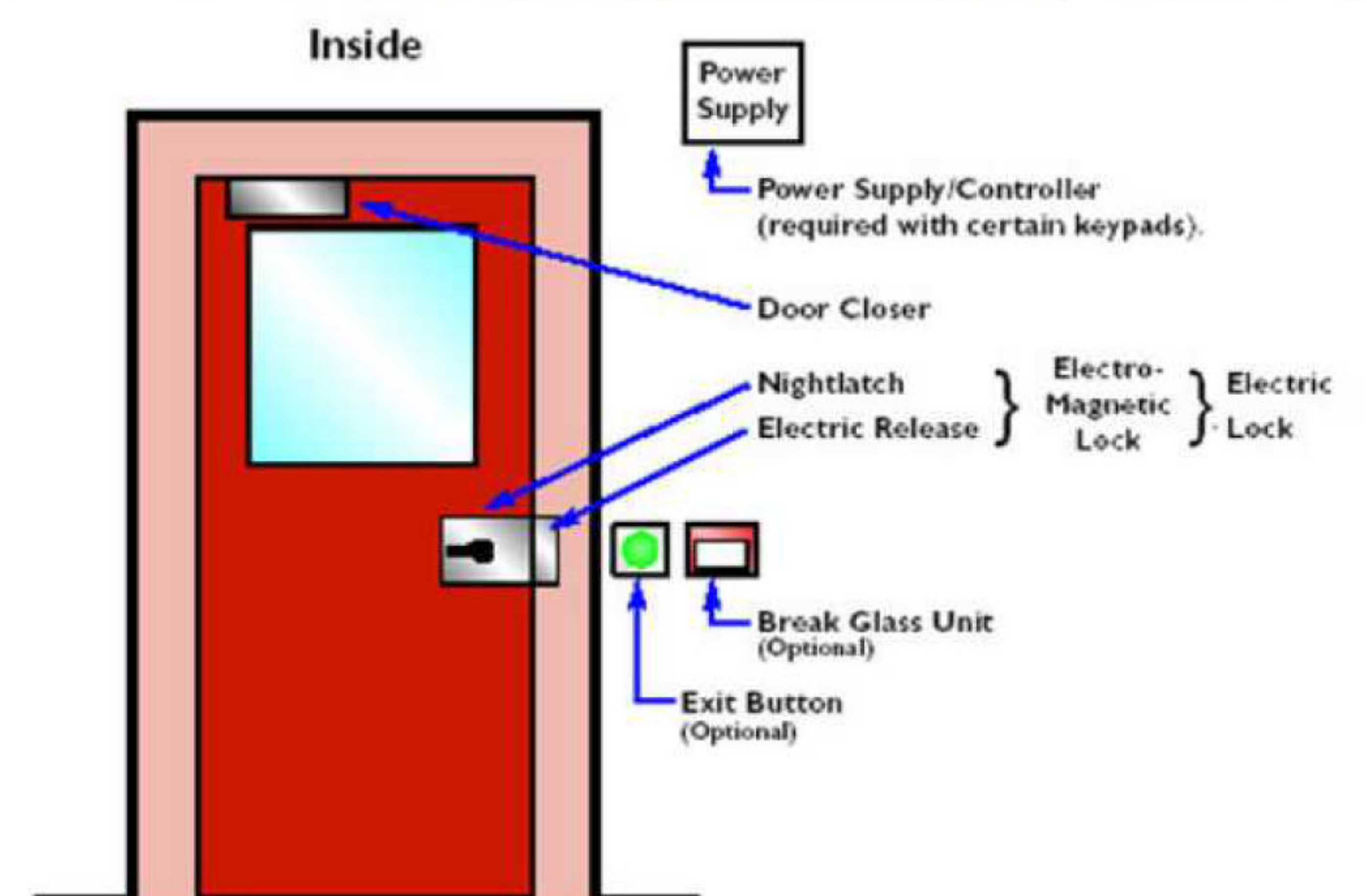
Model : Break Glass Fire Emergency Exit Release
